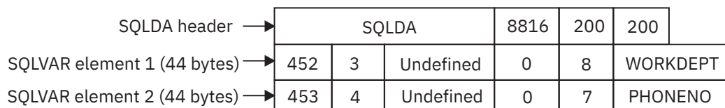
Figure 32. Contents of FULSQLDA after executing DESCRIBE
